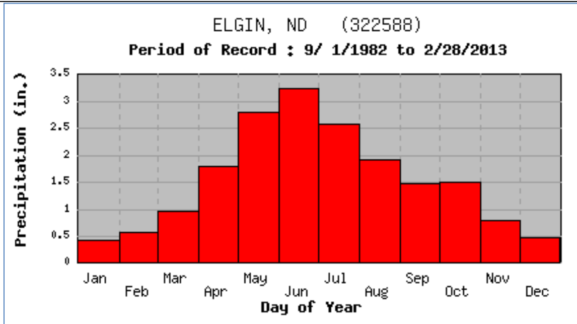
Figure 5. Monthly Precipitation for the Weather Station Located at Elgin, ND (High Plains Regional Climate Center).
