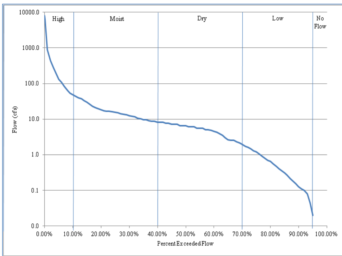
Figure 9. Flow Duration Curve for Cannonball River Monitoring Site 385136.
