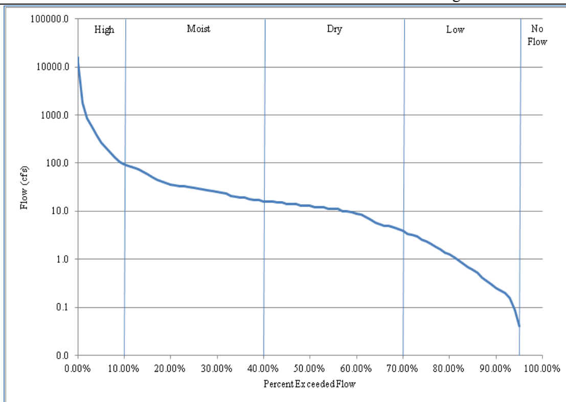
Figure 8. Flow Duration Curve for the Cannonball River Monitoring Site 380105.
