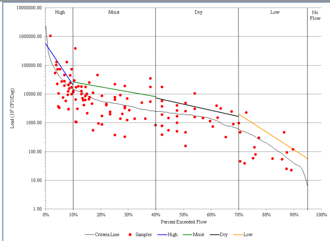
Figure 11. E. coli Bacteria Load Duration Curve for Cannonball River Monitoring Site 385136.
