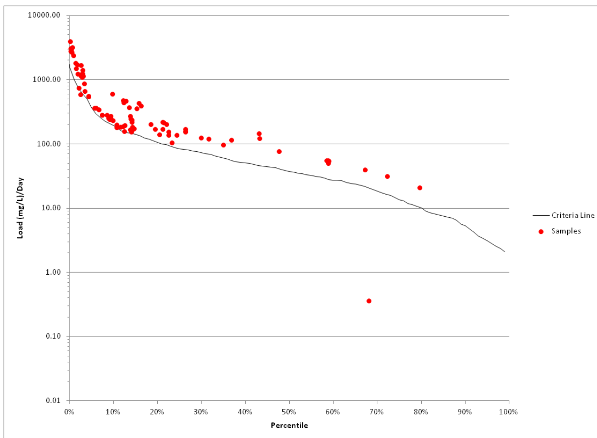
Figure 10. Total Phosphorus Load Duration Curve for the Sheyenne River Monitoring Station 380153 (The curve reflects flow data from 1990-2010).
