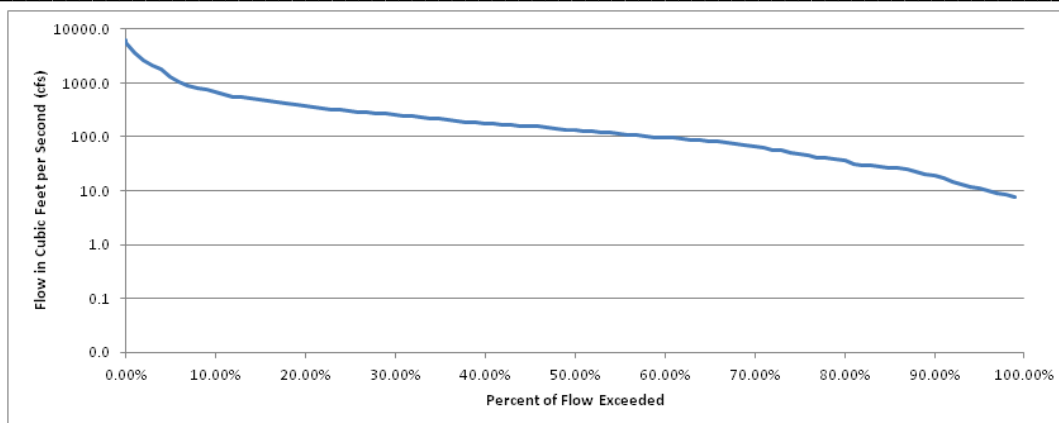
Figure 8. Flow Duration Curve for USGS Gauging Station 05058000.
