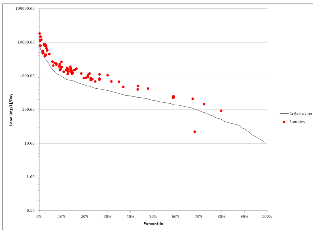
Figure 9. Total Nitrogen Load Duration Curve for the Sheyenne River Monitoring Station 380153 (The curve reflects flow data from 1990-2010).
