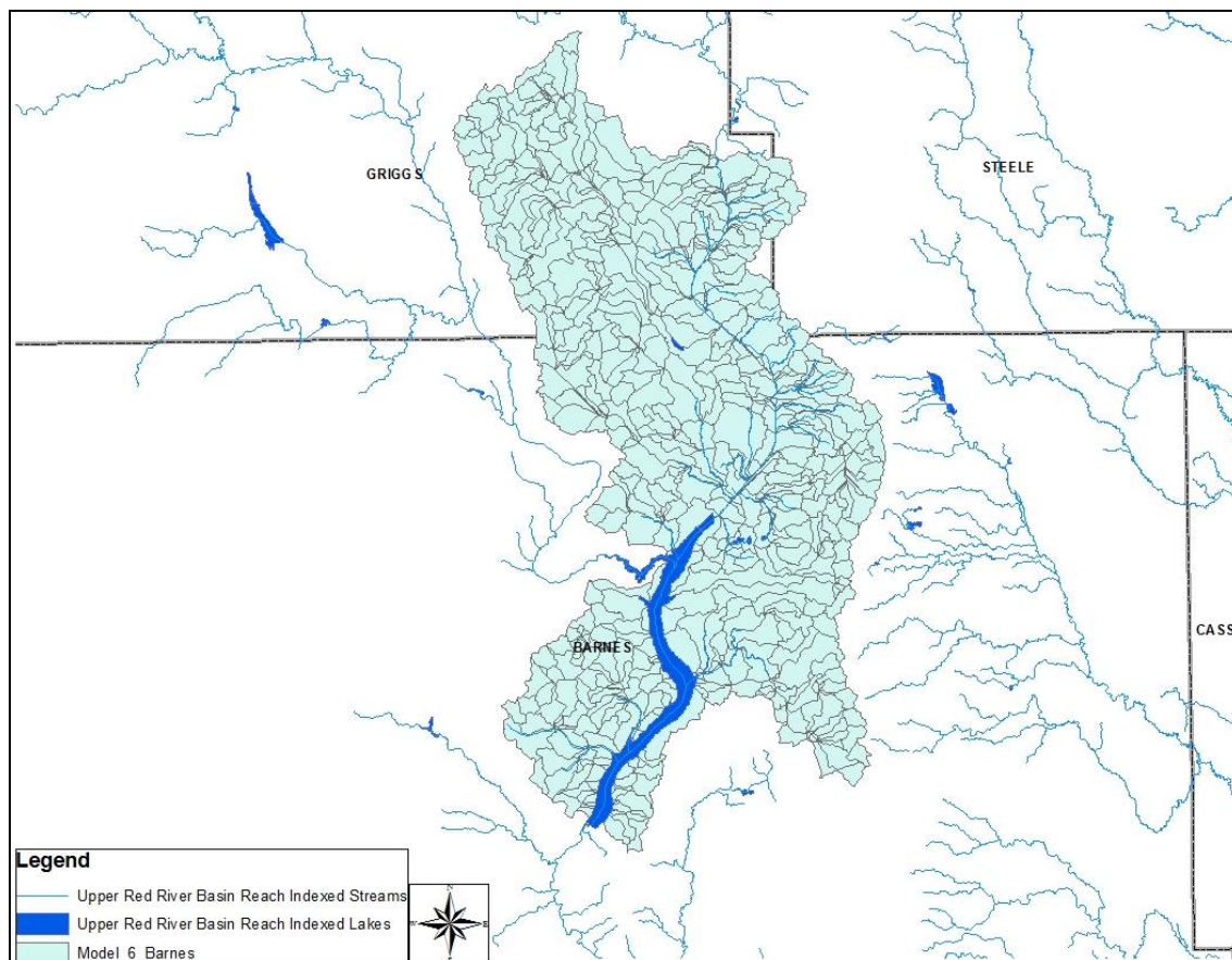
Figure 18. AnnAGNPS Model Watershed Delineation for Barnes Model.
