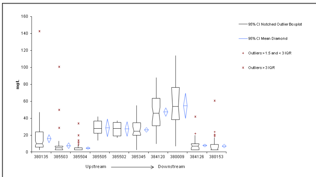
Figure 17. Box and Whisker Plot of Total Suspended Solids for all Water Quality Sampling Sites in the Upper and Middle Sheyenne River.
