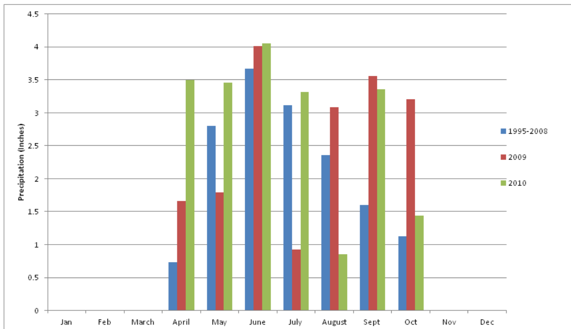
Figure 5. Monthly Precipitation for NDAWN Weather Station Located Near Crary, ND.
