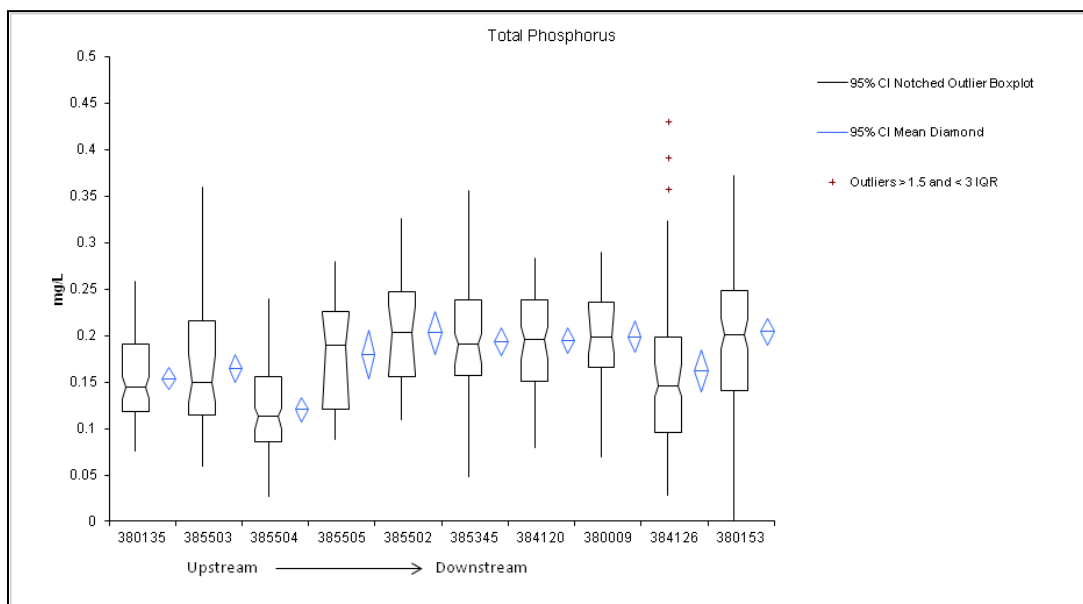
Figure 16. Box and Whisker Plot of Total Phosphorus for all Water Quality Sampling Sites in the Upper and Middle Sheyenne River.
