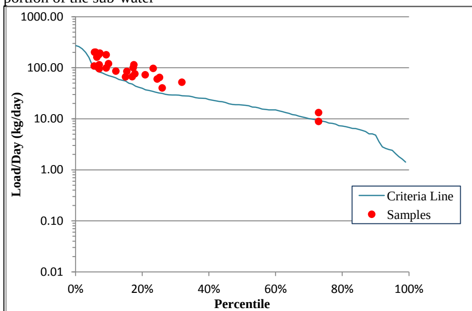
Figure 14. Total Phosphorus Load Duration Curve for the Sheyenne River Monitoring Station 385502 (The curve reflects flow data from 2005 to 2010).
