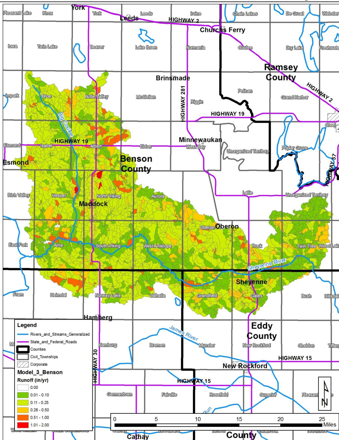
Figure 21. AnnAGNPS Model Predicted Water Runoff for the Benson Model (Moore Engineering, 2010).
