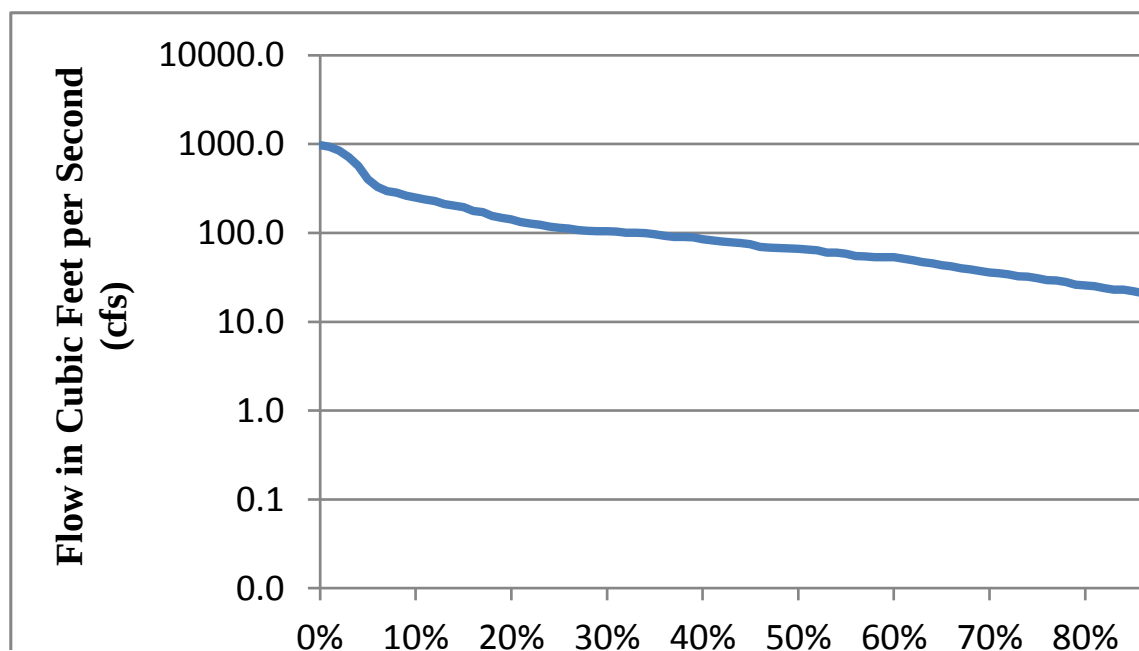
Figure 10. Flow Duration Curve for USGS Gauging Station 05055400.
