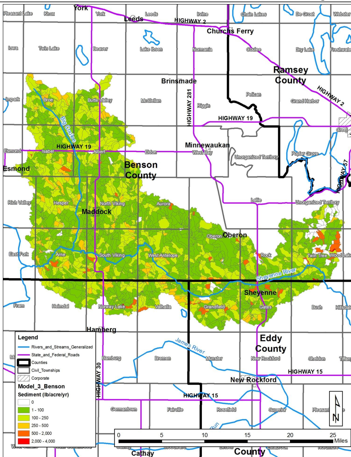
Figure 24. AnnAGNPS Model Predicted Sediment Yield for the Benson Model (Moore Engineering, 2010).
