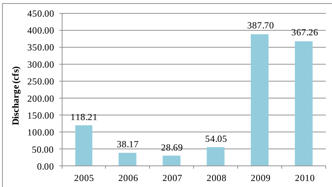
Figure 8. Mean Annual Discharge at the USGS Gauging Station (05055400) on the Sheyenne River near Brennan, ND.
