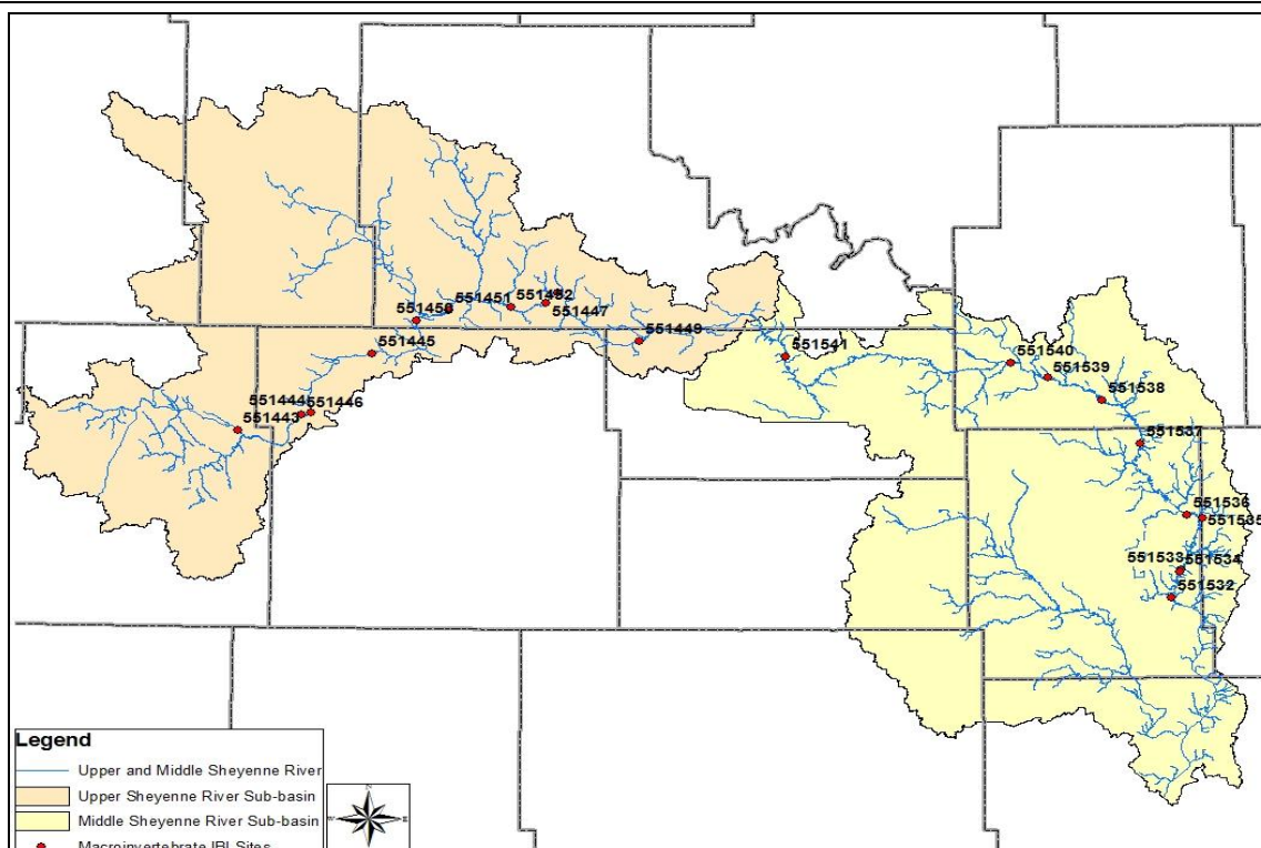
Figure 19. Macroinvertebrate Index of Biotic Integrity Sites on the Upper and Middle Sheyenne River.
