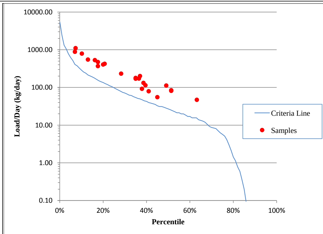
Figure 11. Total Nitrogen Load Duration Curve for the Sheyenne River Monitoring Station 385505 (The curve reflects flow data from 2004 to 2010).
