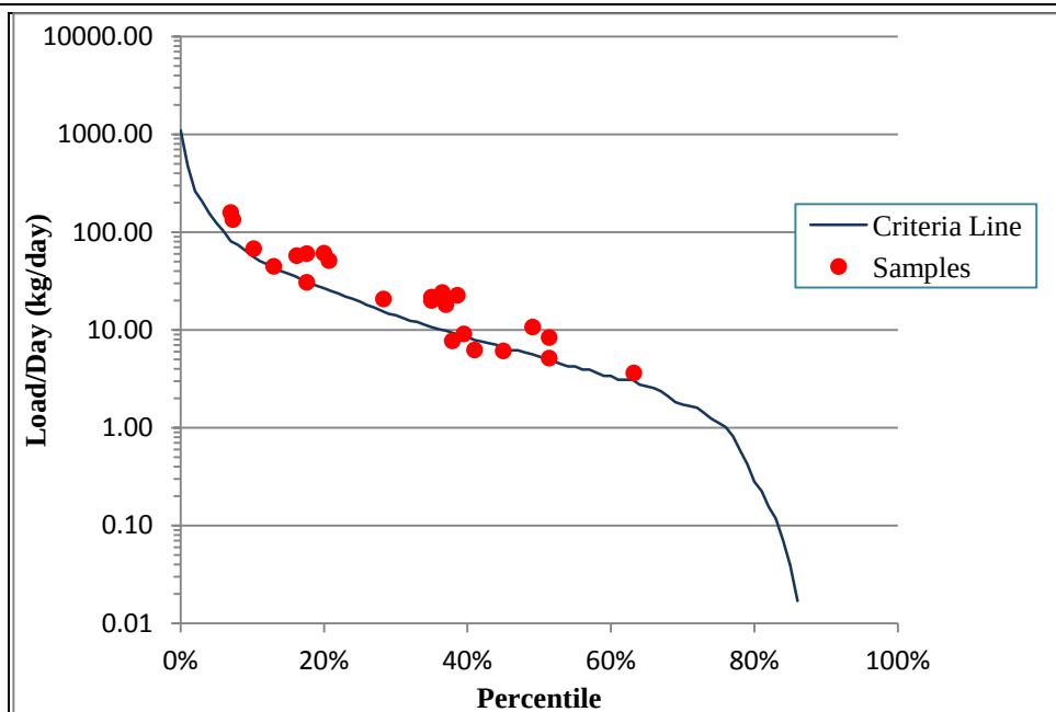
Figure 13. Total Phosphorus Load Duration Curve for the Sheyenne River Monitoring Station 385505 (The curve reflects flow data from 2004 to 2010).
