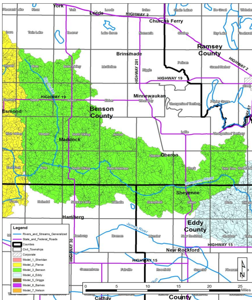
Figure 20. AnnAGNPS Model Watershed Delineation for the Benson Model.
