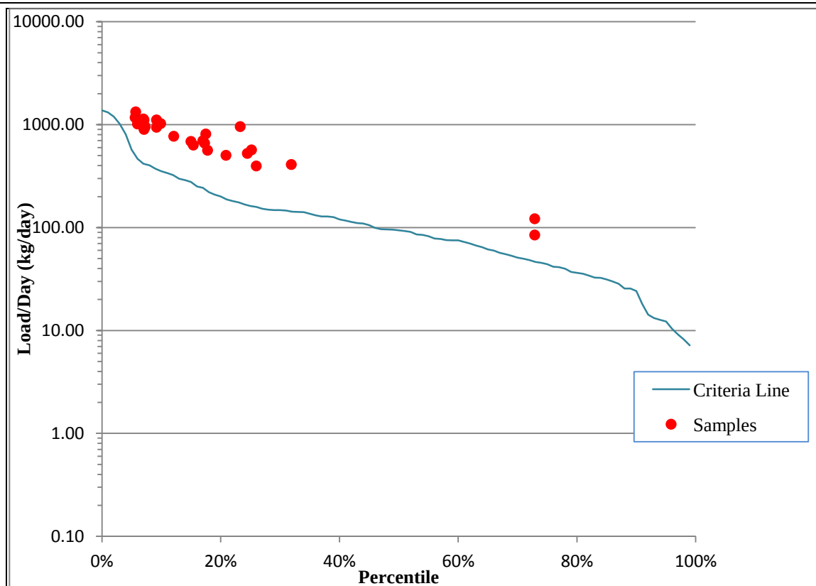
Figure 12. Total Nitrogen Load Duration Curve for the Sheyenne River Monitoring Station 385502 (The curve reflects flow data from 2005 to 2010).
