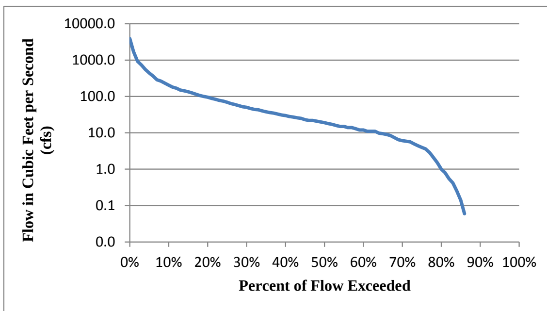
Figure 9. Flow Duration Curve for USGS Gauging Station 05055300.
