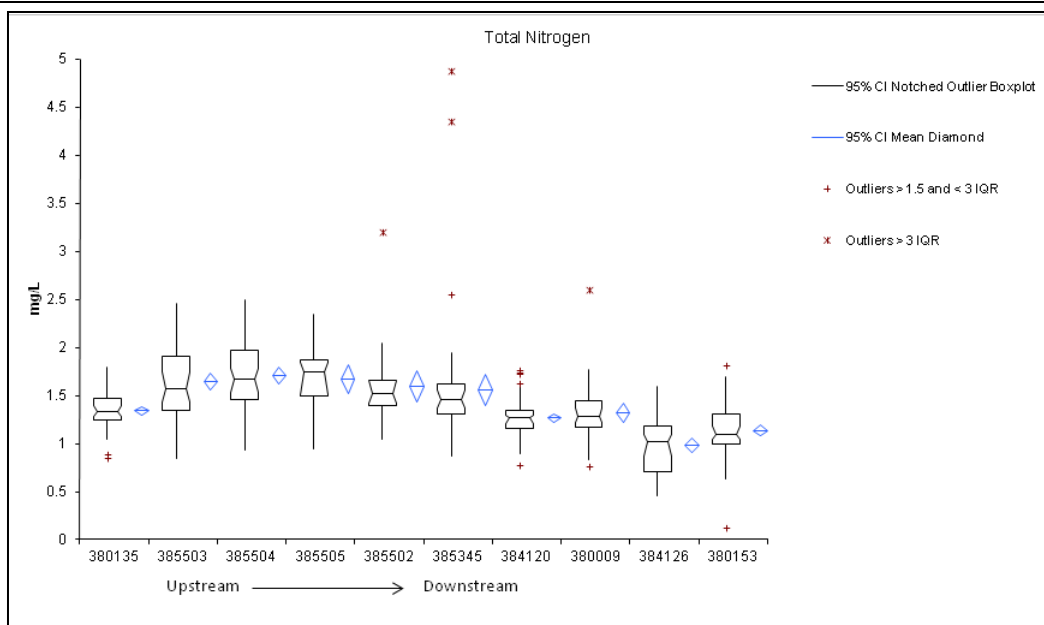
Figure 15. Box and Whisker Plot of Total Nitrogen for all Water Quality Sampling Sites in the Upper and Middle Sheyenne River.
