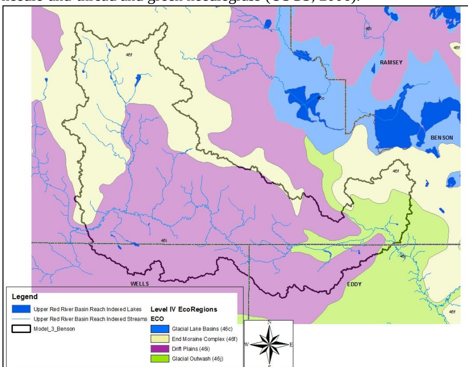
Figure 4. Level IV Ecoregions in the Benson Model Watershed.
