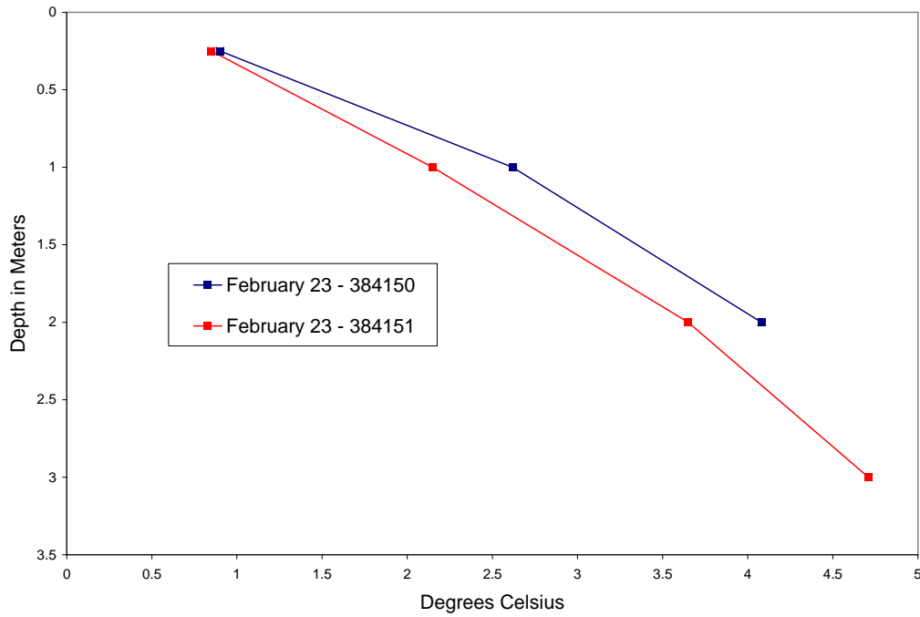
Figure 8. February 23, 1998 Temperature Profiles
