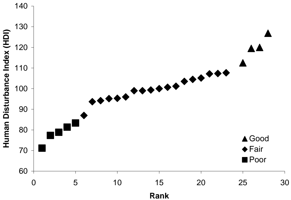
Figure 2. Distribution of the Human Disturbance Index Ranked from Lowest to Highest Score.
