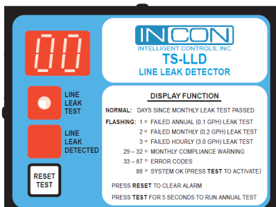
InCon line leak detector display
