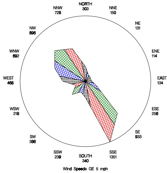
Bear Paw – MGP #5 Wind Direction Star Chart during 2005
