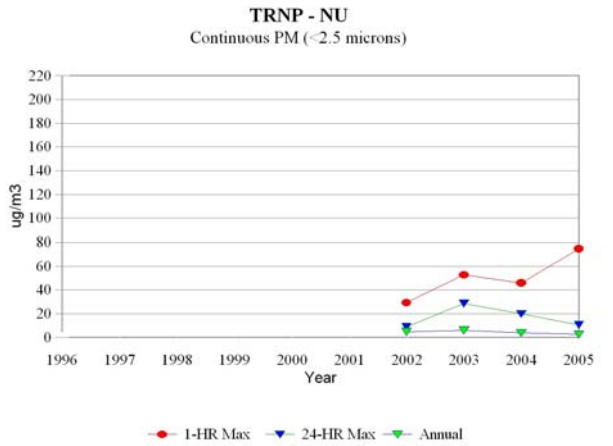
Figure A4-11 TRNP - NU Trends
