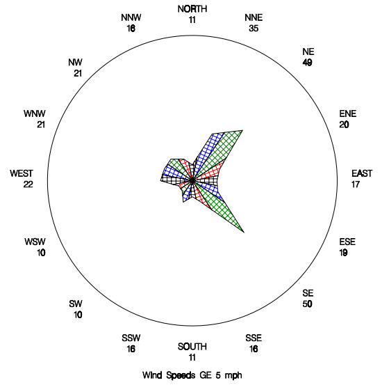
Percent of Time SO2 Detected for a Given Wind Sector for Hannover during 2005
