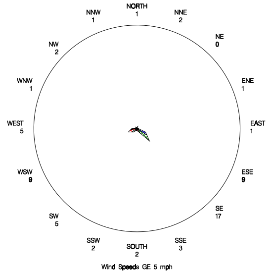
Percent of Time SO2 Detected for a Given Wind Sector for Fargo NW during 2005
