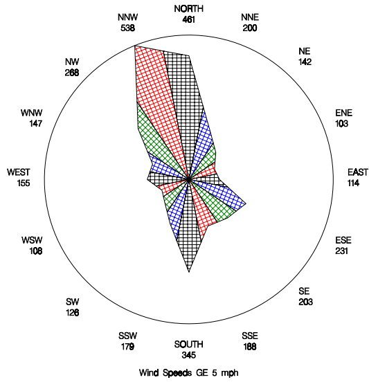
Mandan NW – SPM Wind Direction Star Chart during 2005
