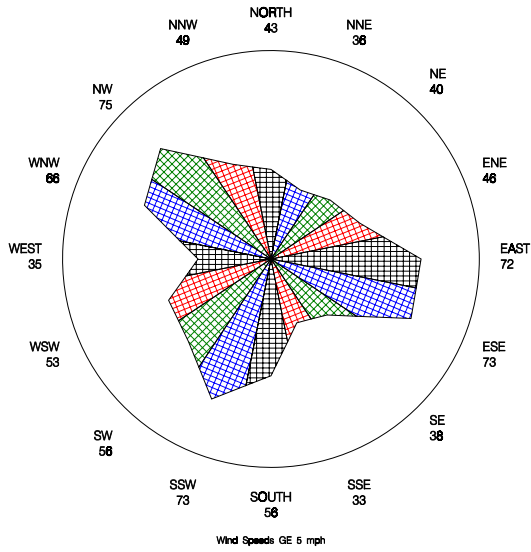
Percent of Time SO2 Detected for a Given Wind Sector for DGC #16 during 2005
