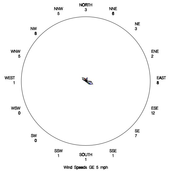
Percent of Time SO2 Detected for a Given Wind Sector for Bear Paw – MGP #5 during 2005
