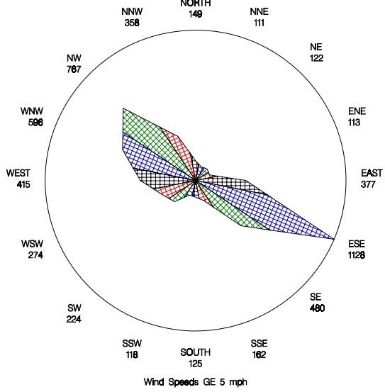
Bear Paw – MGP #5 Wind Direction Star Chart during 2005
