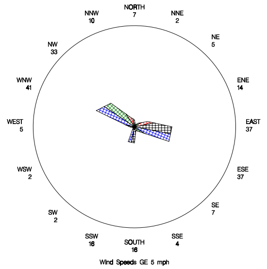
Percent of Time SO2 Detected for a Given Wind Sector for DGC #14 during 2005
