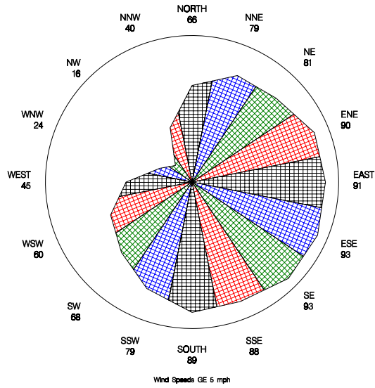
Percent of Time NO2 Detected for a Given Wind Sector for Fargo NW during 2005
