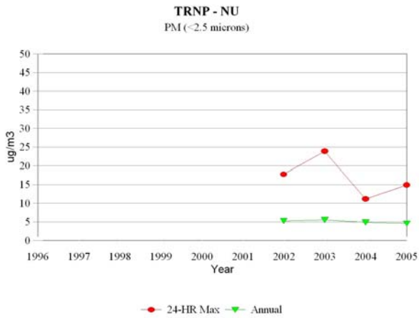
Figure A4-11 TRNP - NU Trends
