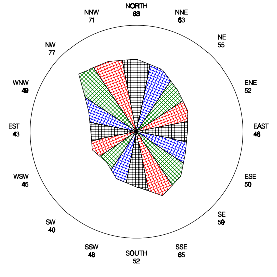
Percent of Time NH3 Detected for a Given Wind Sector for Beulah – North during 2005
