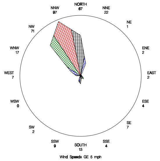
Percent of Time SO2 Detected for a Given Wind Sector for Mandan NW – SPM during 2005
