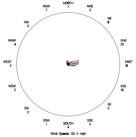
Percent of Time SO2 Detected for a Given Wind Sector for Dunn Center during 2005
