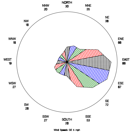
Percent of Time NO2 Detected for a Given Wind Sector for DGC #17 during 2005
