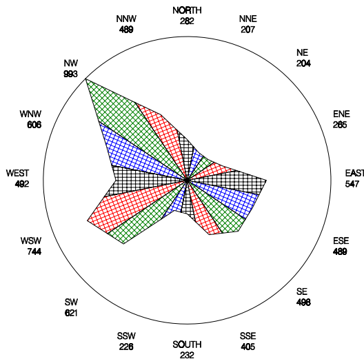
Percent of Time NO2 Detected for a Given Wind Sector for DGC #12 during 2005
