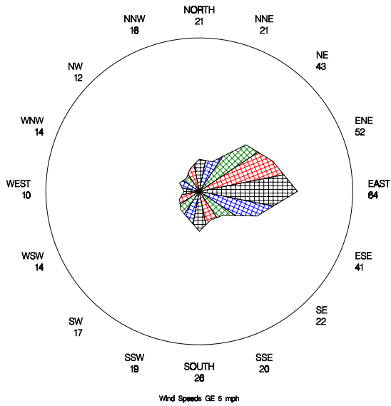
Percent of Time NO2 Detected for a Given Wind Sector for Dunn Center during 2005
