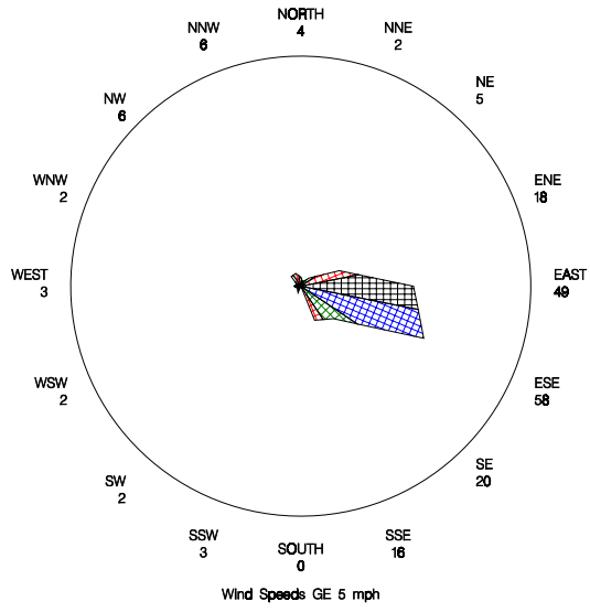
Percent of Time SO2 Detected for a Given Wind Sector for DGC #17 during 2005
