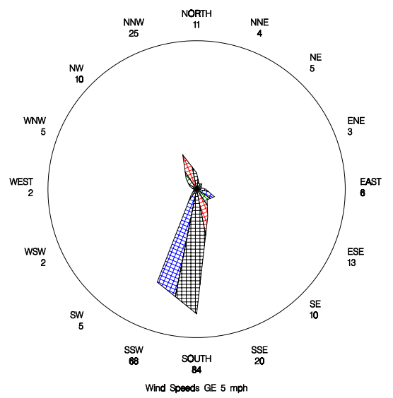
Percent of Time SO2 Detected for a Given Wind Sector for Amerada Hess – Tioga #1 during 2005
