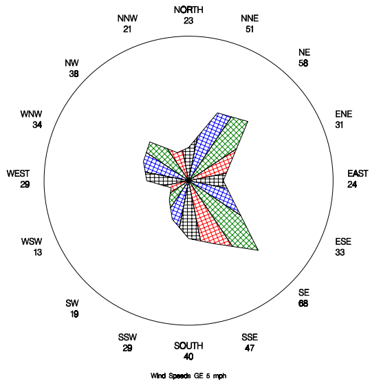
Percent of Time NO2 Detected for a Given Wind Sector for Hannover during 2005
