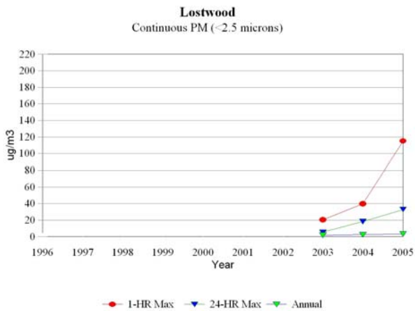
Figure A4-9 Lostwood NWR Trends
