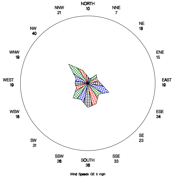
Percent of Time NO2 Detected for a Given Wind Sector for Lostwood NWR during 2005
