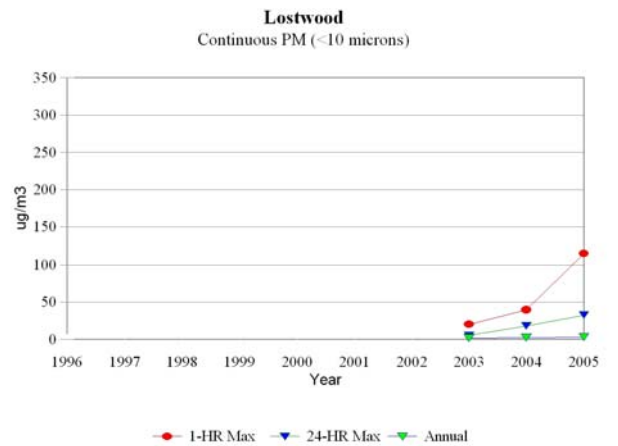
Figure A4-9 Lostwood NWR Trends
