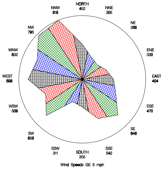
Percent of Time NO2 Detected for a Given Wind Sector for Beulah – North during 2005
