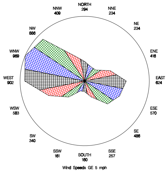
Percent of Time SO2 Detected for a Given Wind Sector for Amerada Hess – Tioga #3 during 2005
