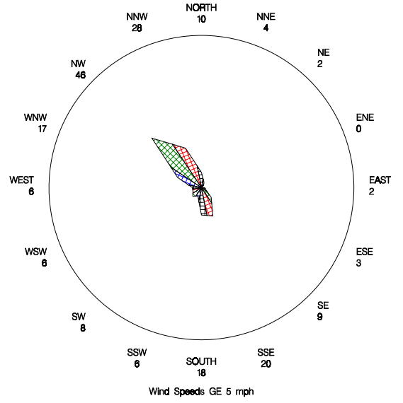
Percent of Time SO2 Detected for a Given Wind Sector for Lostwood NWR during 2005
