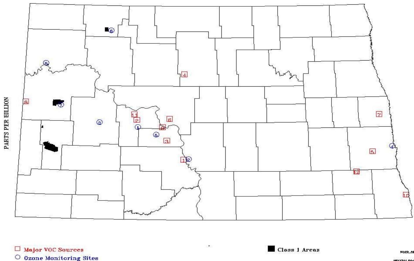
Figure 8 Major VOC Sources
