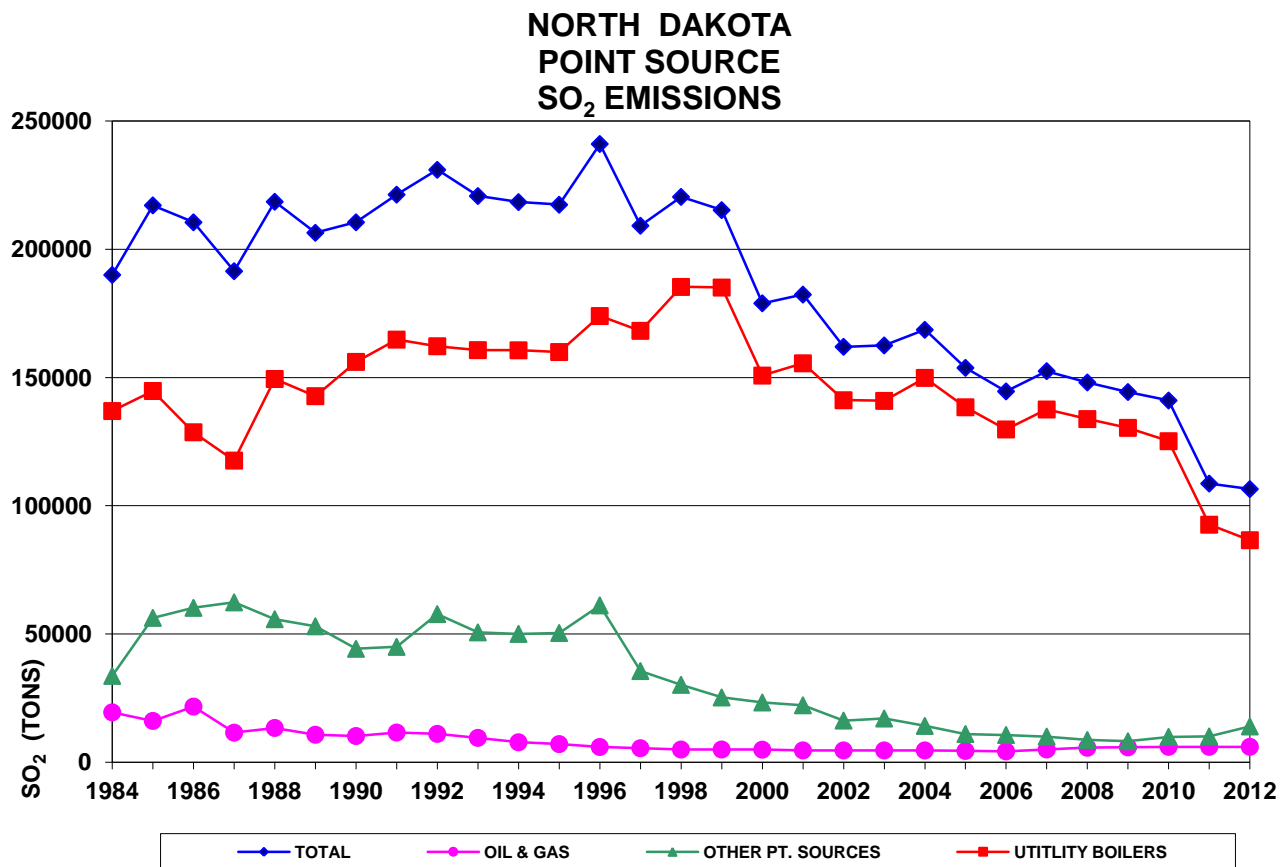
Figure 2A Annual Sulfur Dioxide Emissions
