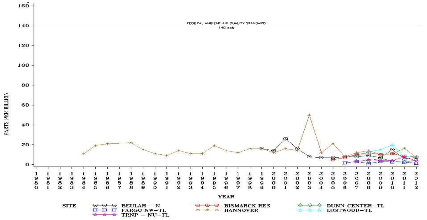
Figure 5 SO 2 Maximum 24-Hour Concentrations
