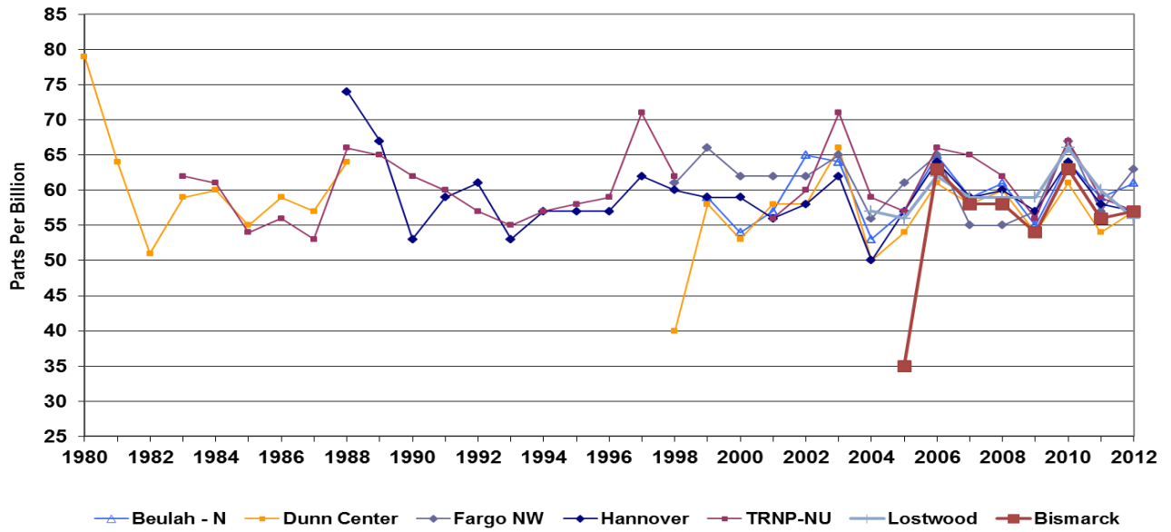
Figure 9 Annual 4 th Highest 8-HR Ozone Concentrations
