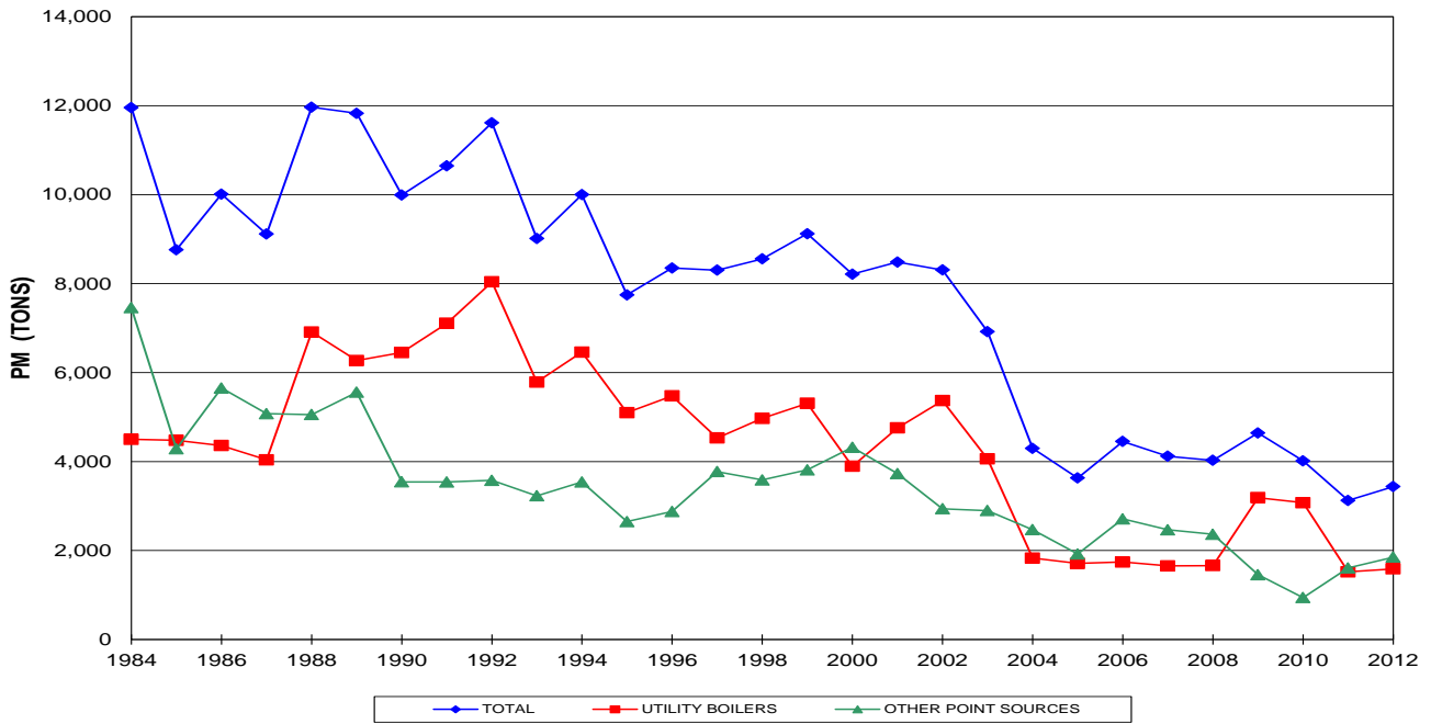
Figure 10A Annual PM Emissions
