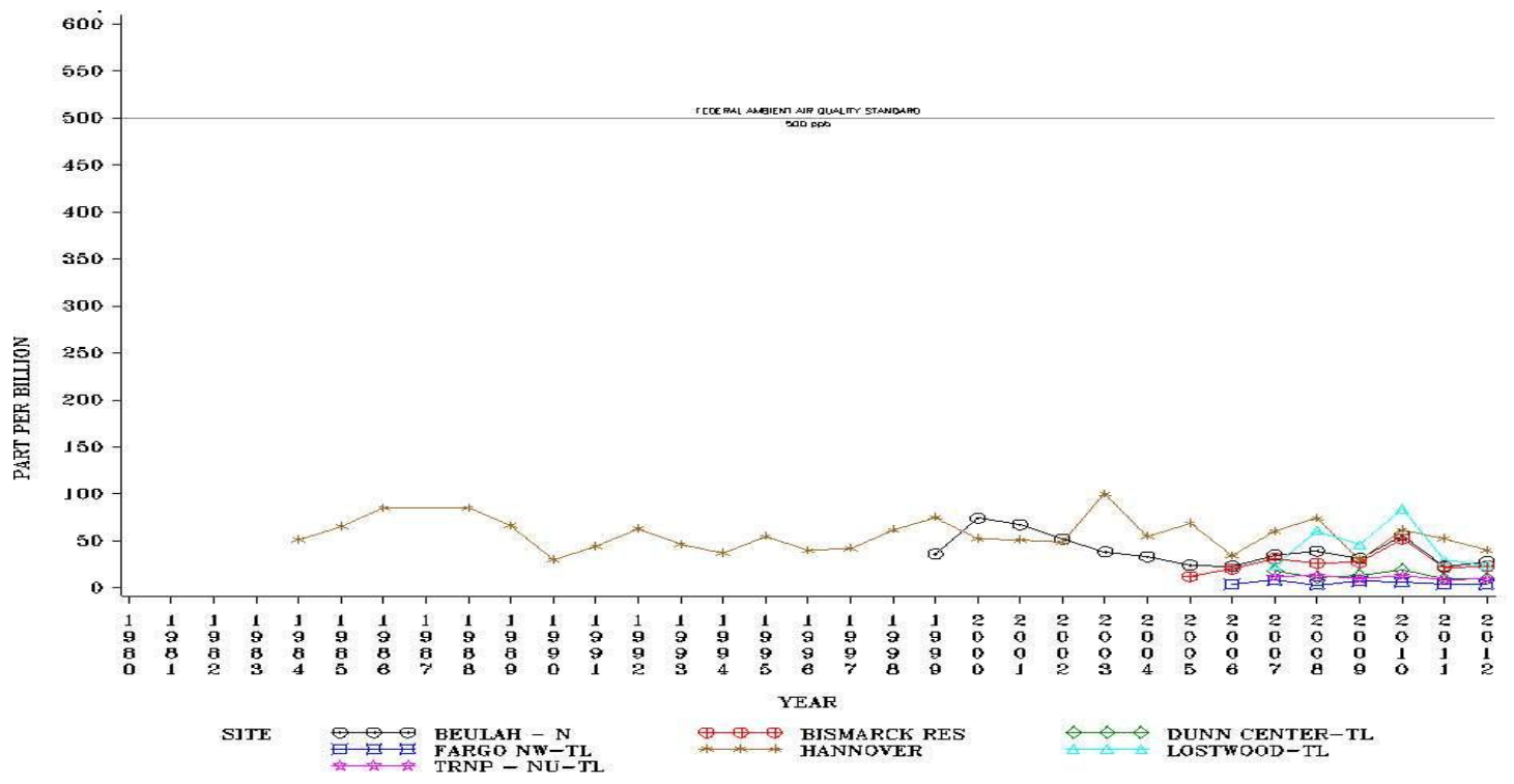
Figure 3 SO 2 Maximum 1-Hour Concentrations
