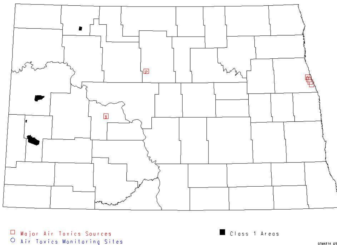
Figure 12 Major Air Toxics Sources
