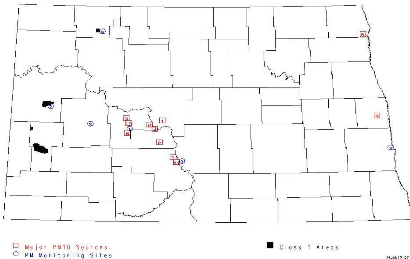
Figure 11 Major PM 10 Sources
