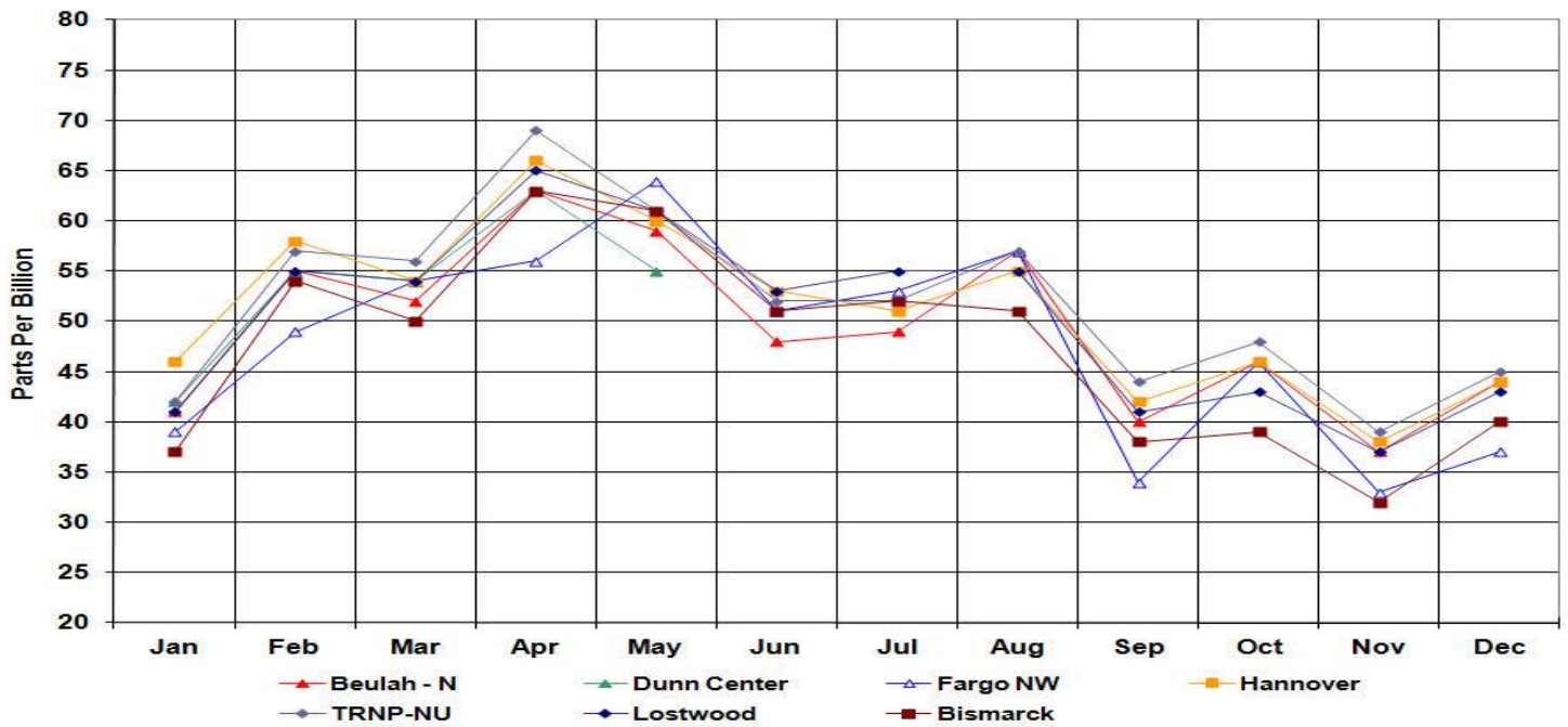
Figure 9 Monthly 4 th Highest Ozone Concentrations
