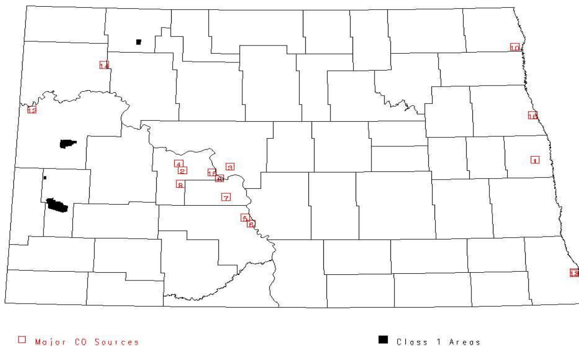
Figure 12 Major CO Sources
