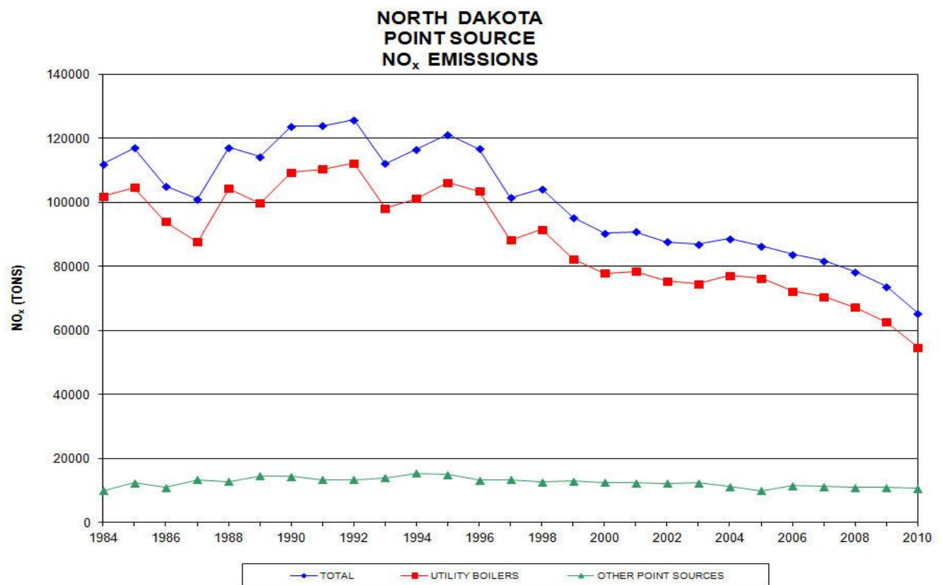
Figure 6A Annual Oxides of Nitrogen Emissions
