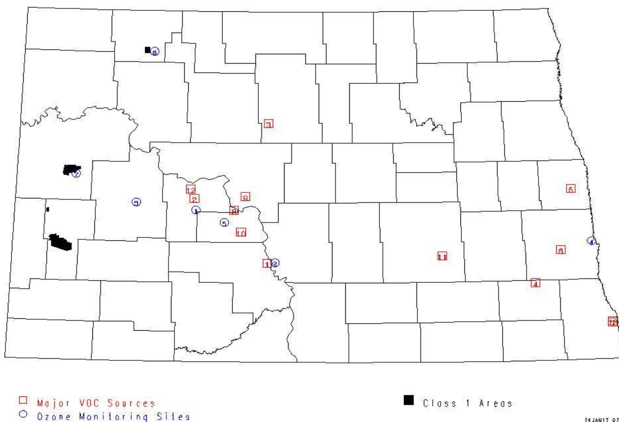
Figure 8 Major VOC Sources
