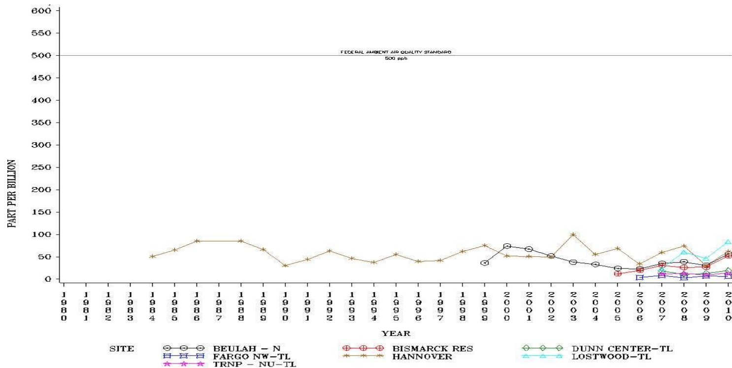
Figure 3 SO 2 Maximum 1-Hour Concentrations
