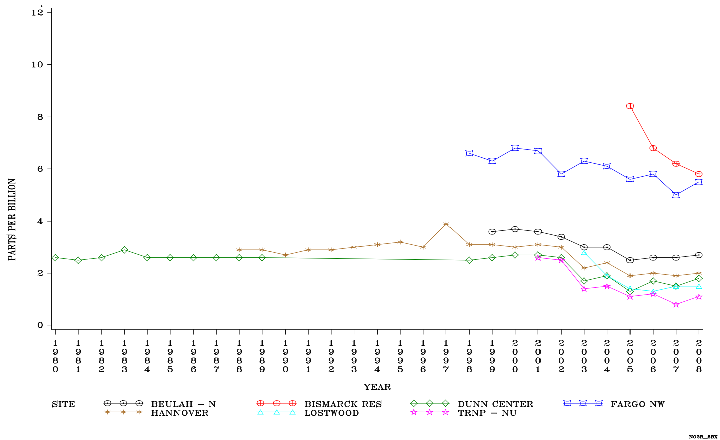
Figure 7 NO 2 Annual Average Concentrations
