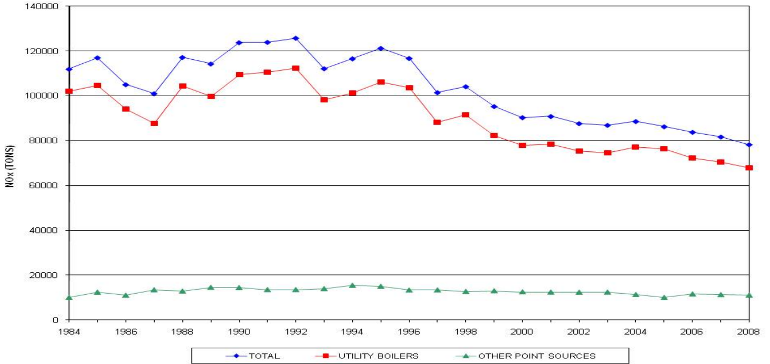
Figure 6A Annual Oxides of Nitrogen Emissions
