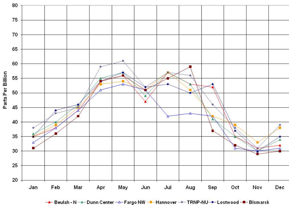
Figure 9 Monthly 4 th Highest Ozone Concentrations
