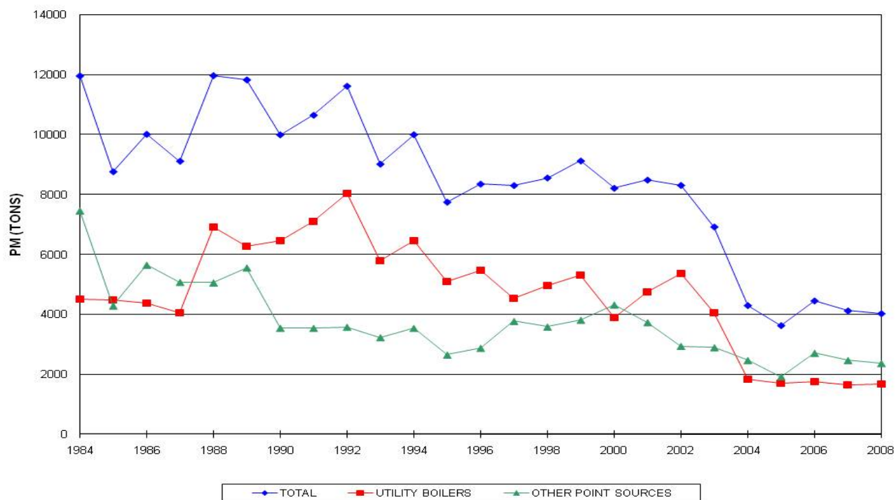
Figure 11A Annual PM Emissions
