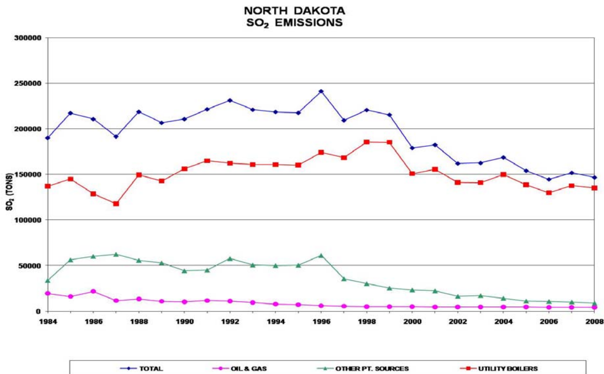
Figure 2A Annual Sulfur Dioxide Emissions
