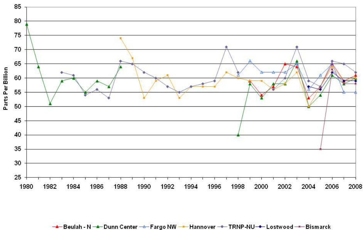
Figure 10 Annual 4 th Highest 8-HR Ozone Concentrations
