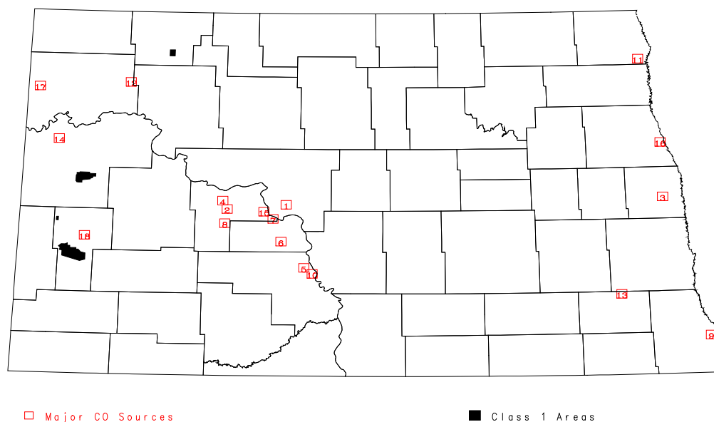
Figure 12 Major CO Sources
