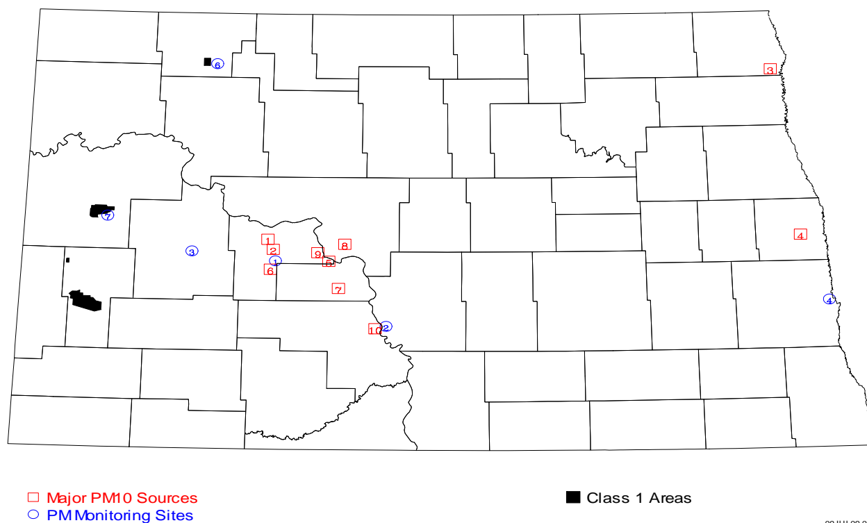
Figure 11 Major PM 10 Sources
