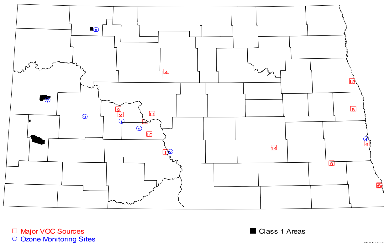
Figure 8 Major VOC Sources
