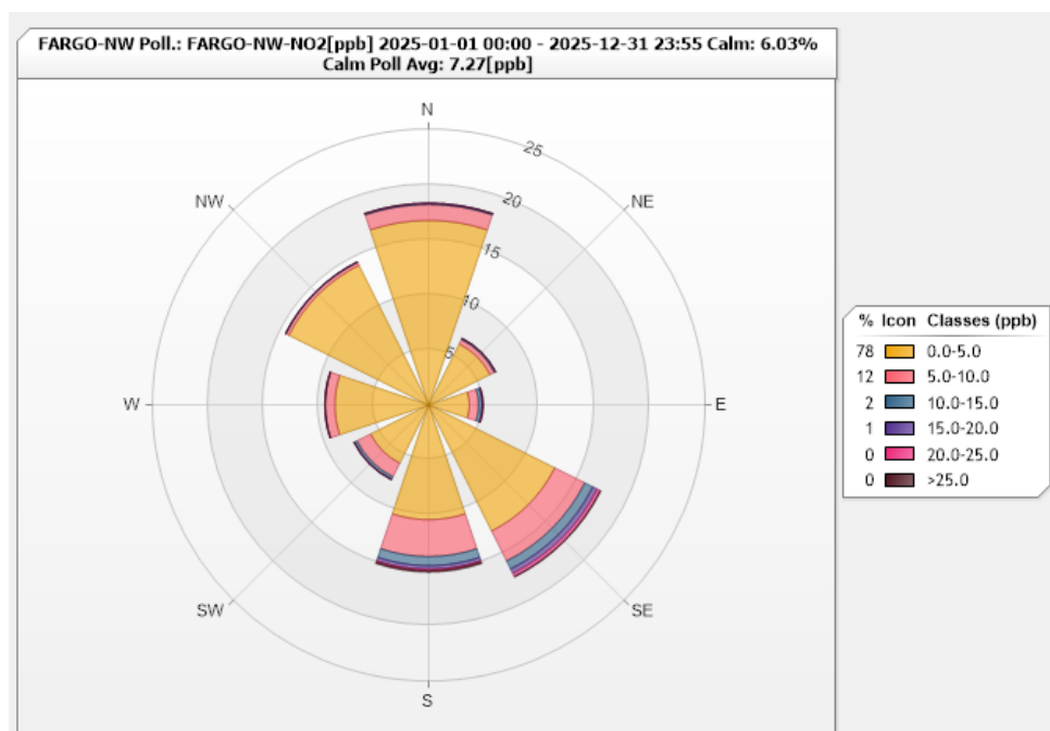
Figure 40. Fargo NO 2 Pollution Rose for 2025
