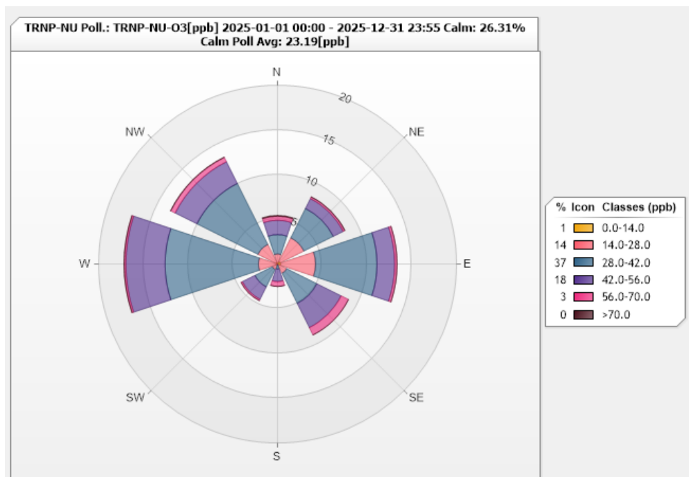
Figure 66. TRNP – North Unit O 3 Pollution Rose for 2025
