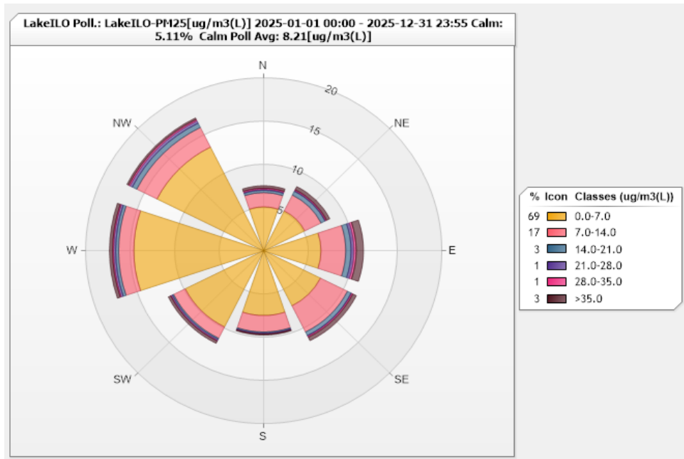
Figure 37. Lake Ilo PM 2.5 Pollution Rose for 2025
