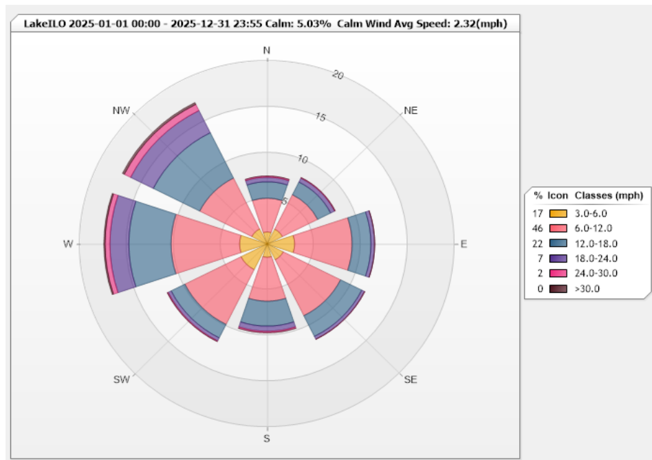
Figure 33. Lake Ilo Wind Rose for 2025
