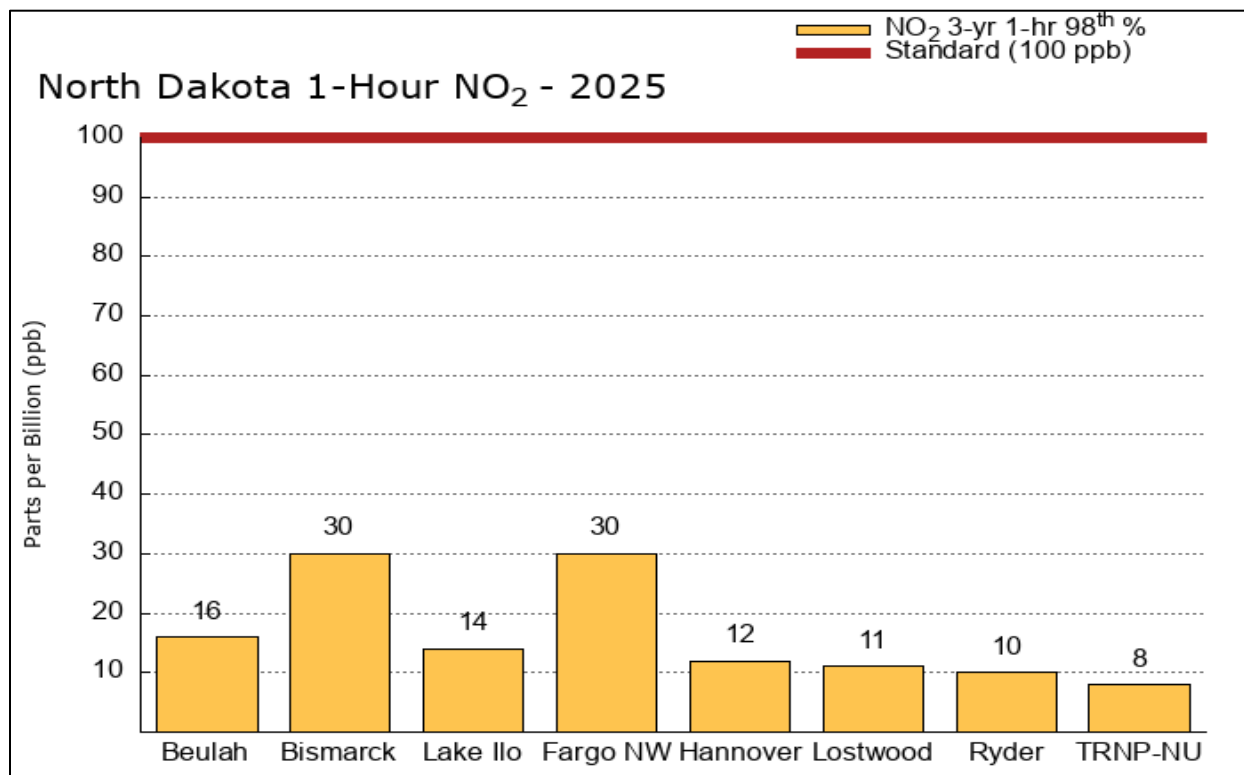
Figure 5. NO 2 Concentrations Compared to the 1-hour Standard (2023-2025)
