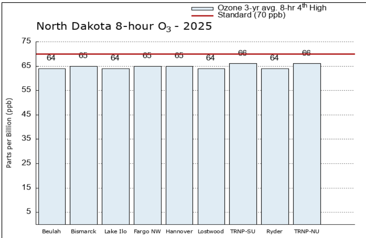
Figure 10. Ozone Concentrations* compared to the 8-hour Standard (2023-2025) * Dataset includes all values (flagged wildfire smoke events included).
