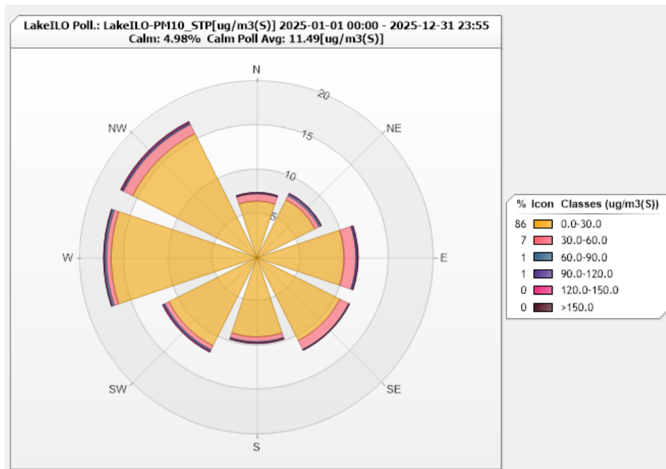
Figure 36. Lake Ilo PM 10 Pollution Rose for 2025
