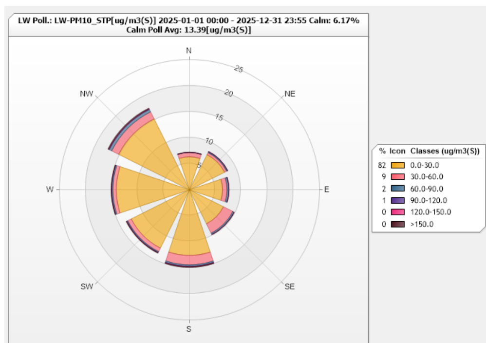
Figure 57. Lostwood PM 10 Pollution Rose for 2025
