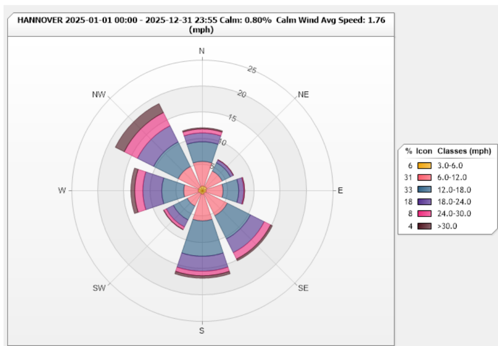
Figure 44. Hannover Wind Rose for 2025
