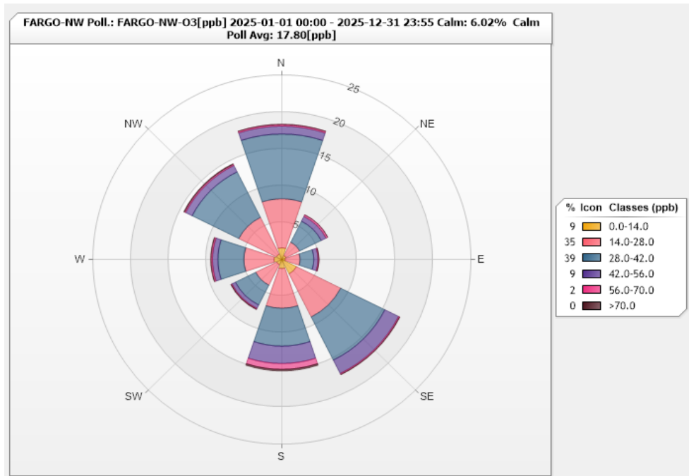
Figure 41. Fargo O 3 Pollution Rose for 2025
