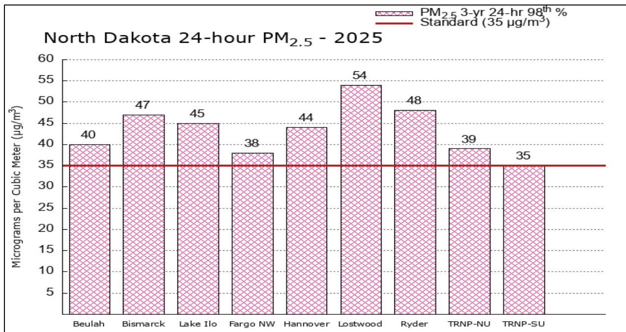
Figure 15. PM 2.5 Concentrations* Compared to the 24-hour Standard (2023-2025) * Dataset includes all values (flagged wildfire smoke events included).
