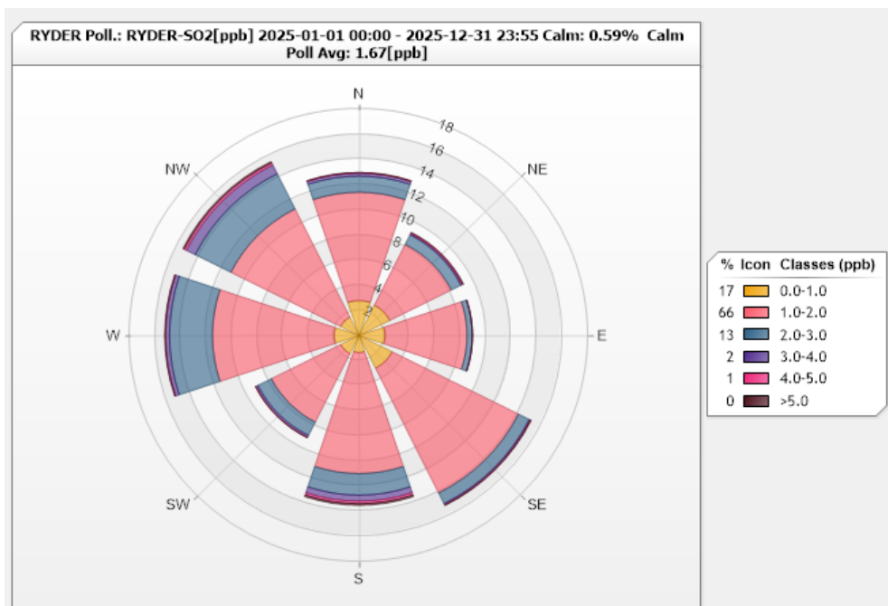
Figure 53. Ryder SO 2 Pollution Rose for 2025
