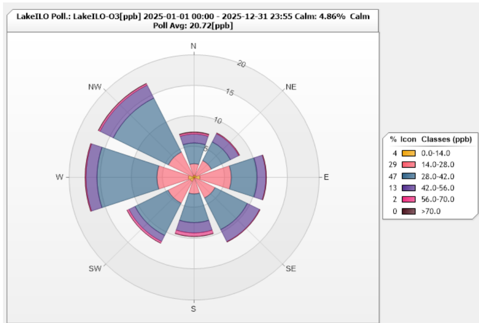
Figure 35. Lake Ilo O 3 Pollution Rose for 2025
