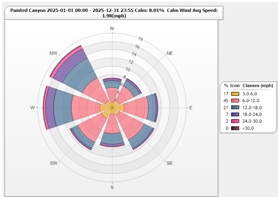
Figure 60. Painted Canyon Wind Rose for 2025
