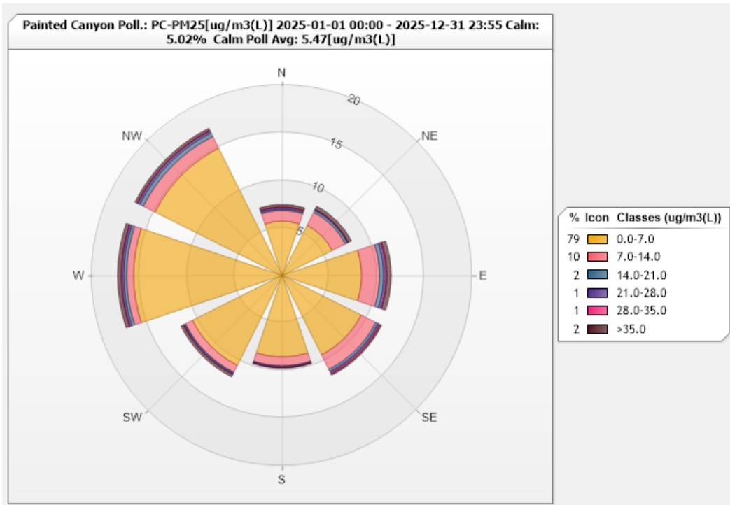
Figure 62. Painted Canyon PM 2.5 Pollution Rose for 2025
