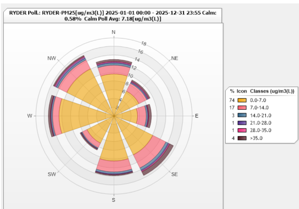
Figure 52. Ryder PM 2.5 Pollution Rose for 2025
