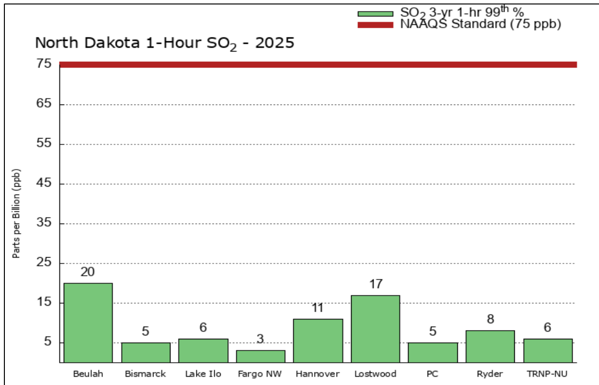
Figure 18. SO 2 Concentrations Compared to the 1-hour Standard (2023-2025)
