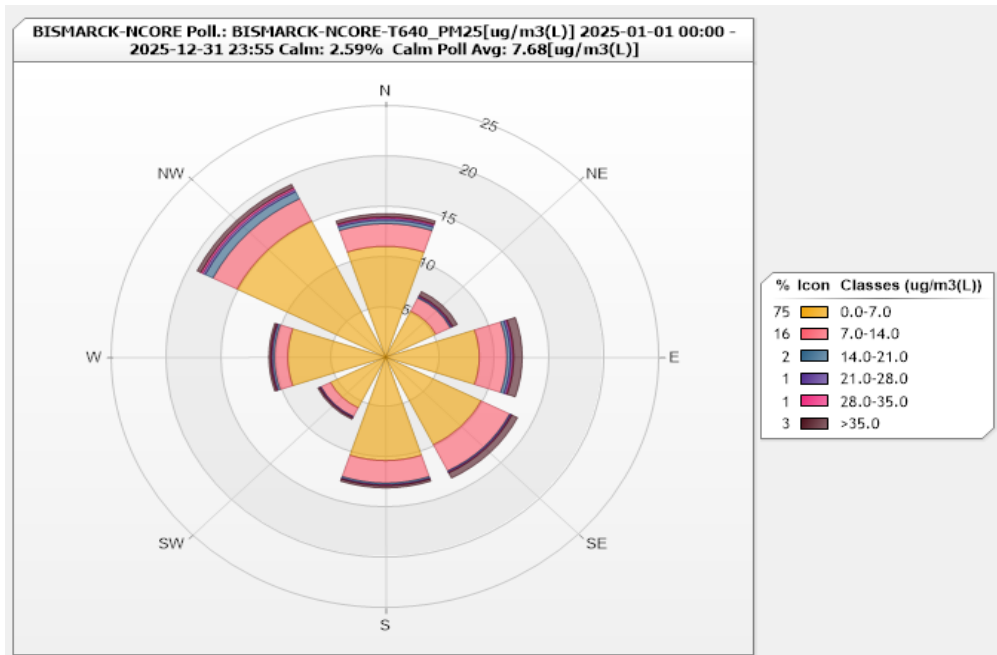
Figure 31. Bismarck PM 2.5 Pollution Rose for 2025
