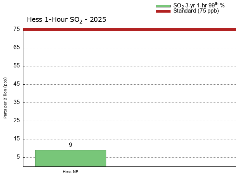
Figure 69. Tioga Gas Plant SO 2 Concentrations Compared to the 1-hour Standard (2023-2025)
