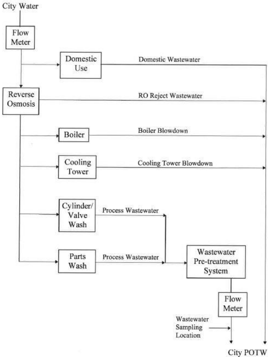
Figure 2 – Process flow diagram for Bobcat Cylinders.
