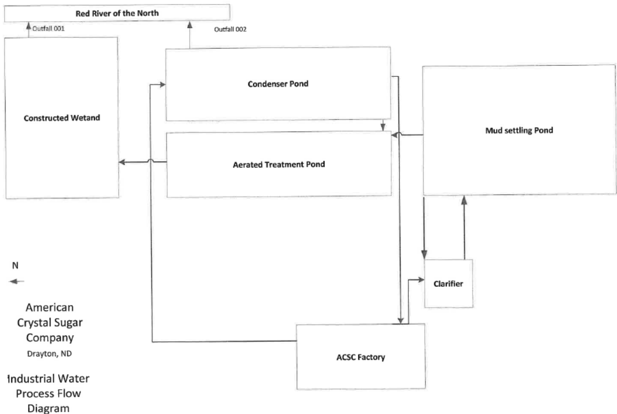
Figure 2 – Flow chart of wastewater for ACS – Drayton. Note: Outfall 001 and Outfall 002 labels are switched.
